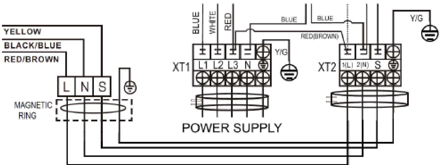
INDOOR UNIT
