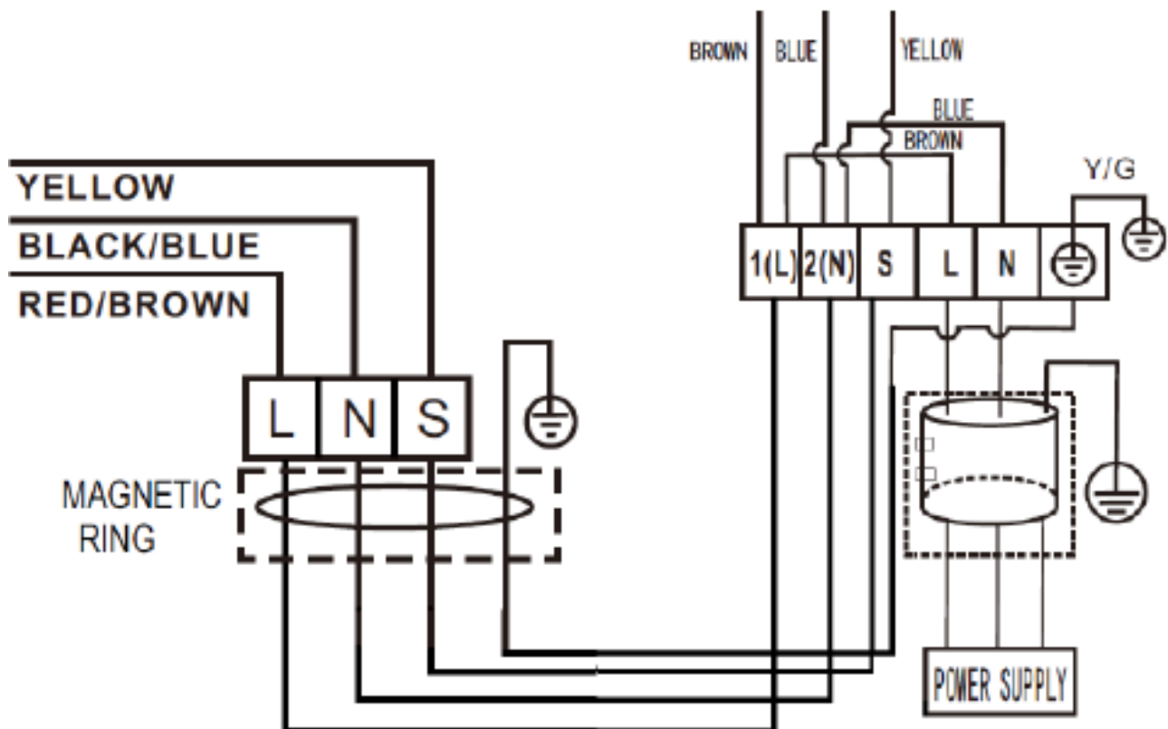
OUTDOOR UNIT
